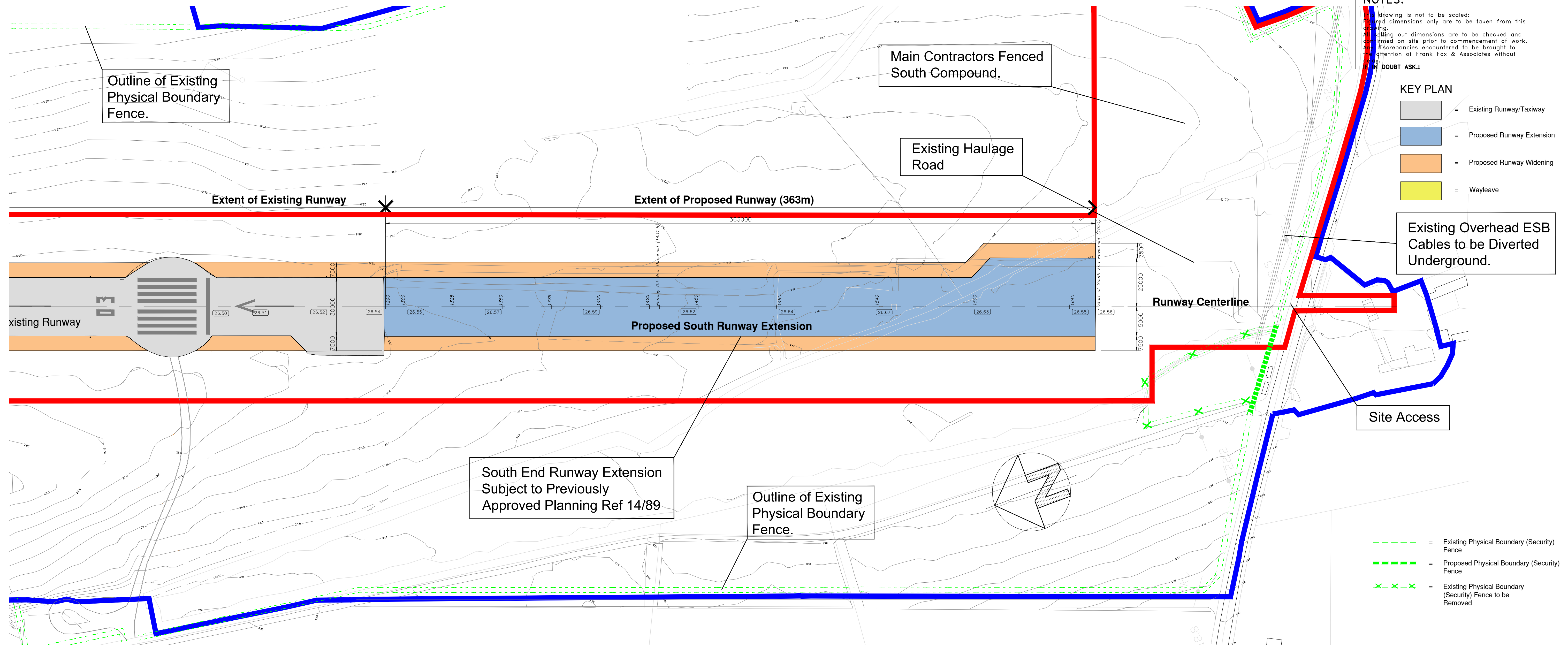
GENERAL ARRANGEMENT SOUTH END RUNWAY EXTENSION LAYOUT
